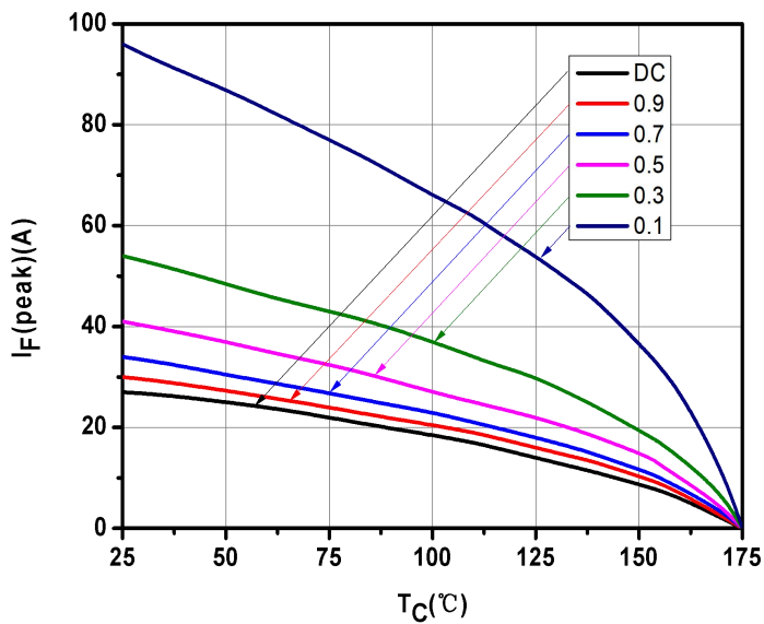
Fig.8-Current Derating
