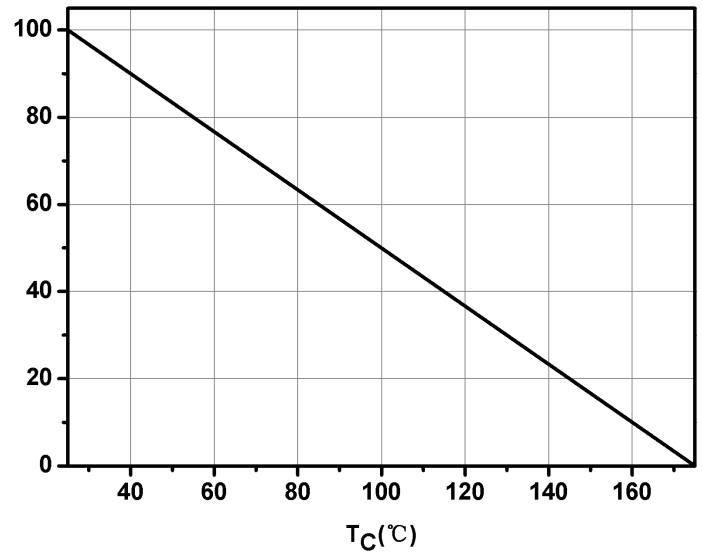
Fig.6-Power Derating
